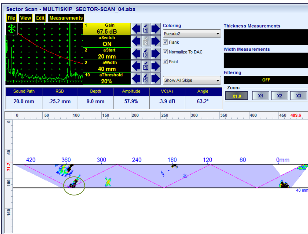
Multi-Skip Sector Scan Coverage of the Medium Thickness Plates, Walls, Bars, Rods, etc
