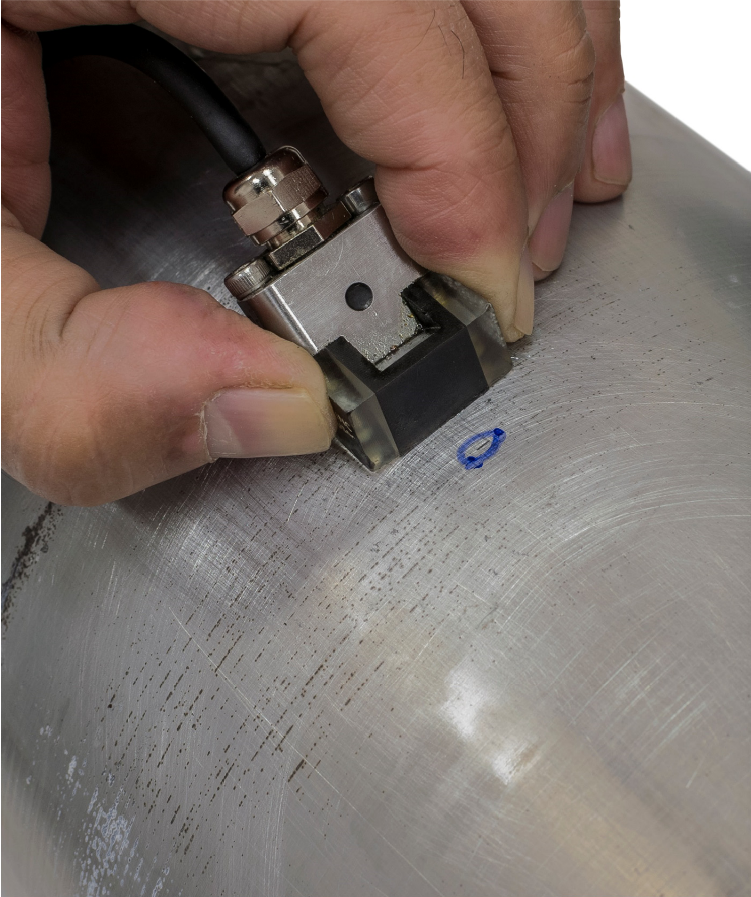
Multi-Skip detection and evaluation of the transversal cracks in the thin walled tubes and tubular parts
